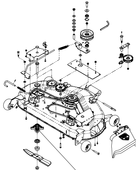
Figure 8 Spindle
