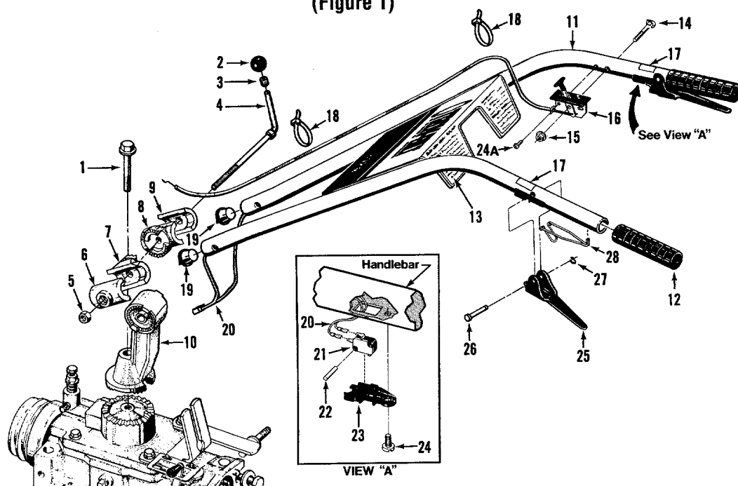
HANDLEBAR ASSEMBLY (Figure 1)
