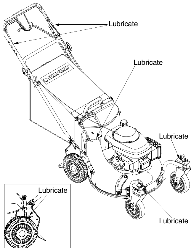
Figure 17: Lubrication Chart
