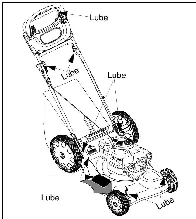
Figure 12: Lubrication Chart
