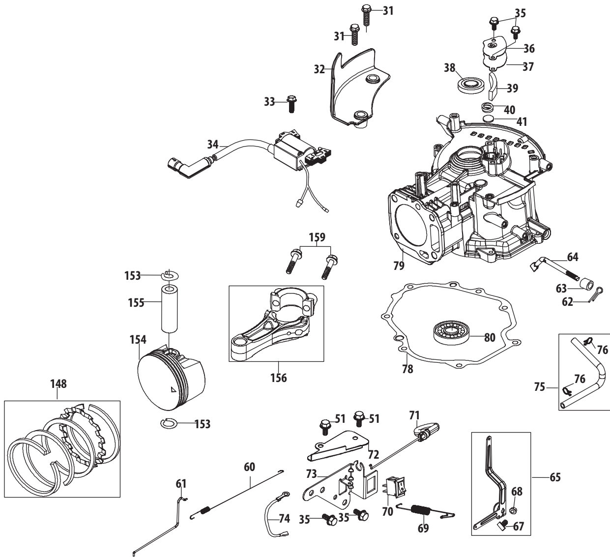
164 - Complete Engine
