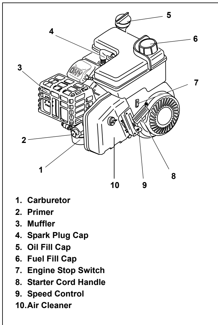
Figure 14. Engine Components
